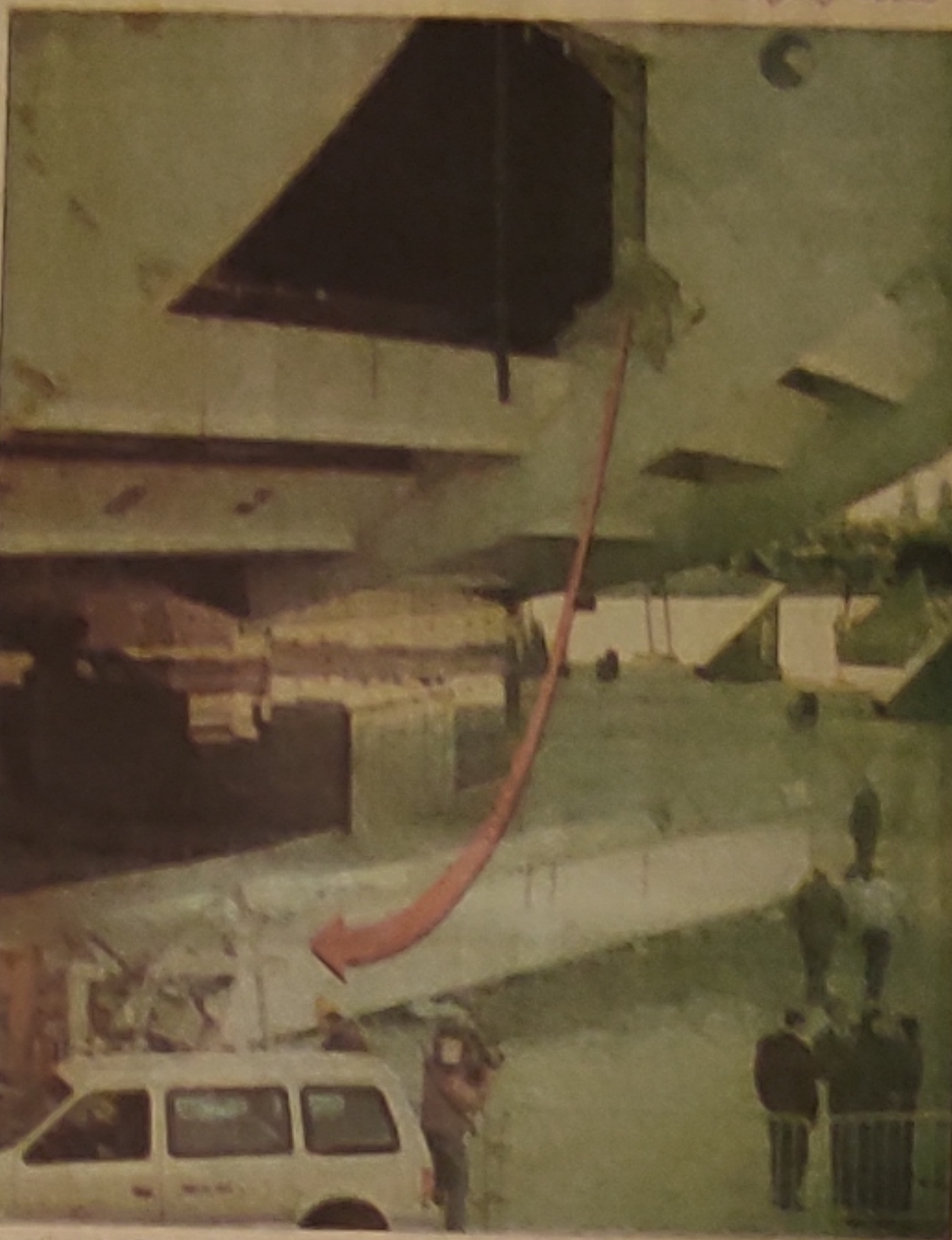
Arrow shows path of 30-tonne, 20-metre-long beam that dropped more than 200 metres at Olympic Stadium yesterday.
