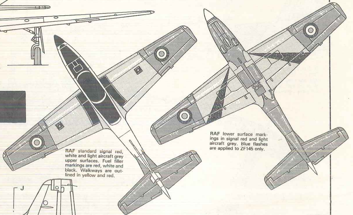
Shorts Tucano T.1 ZF145 of No.7 FTS, RAF during 1990. Standard RAF colouring with roundel blue fuselage and lower wing flashes. Pelican on tail is yellow, black and white.
